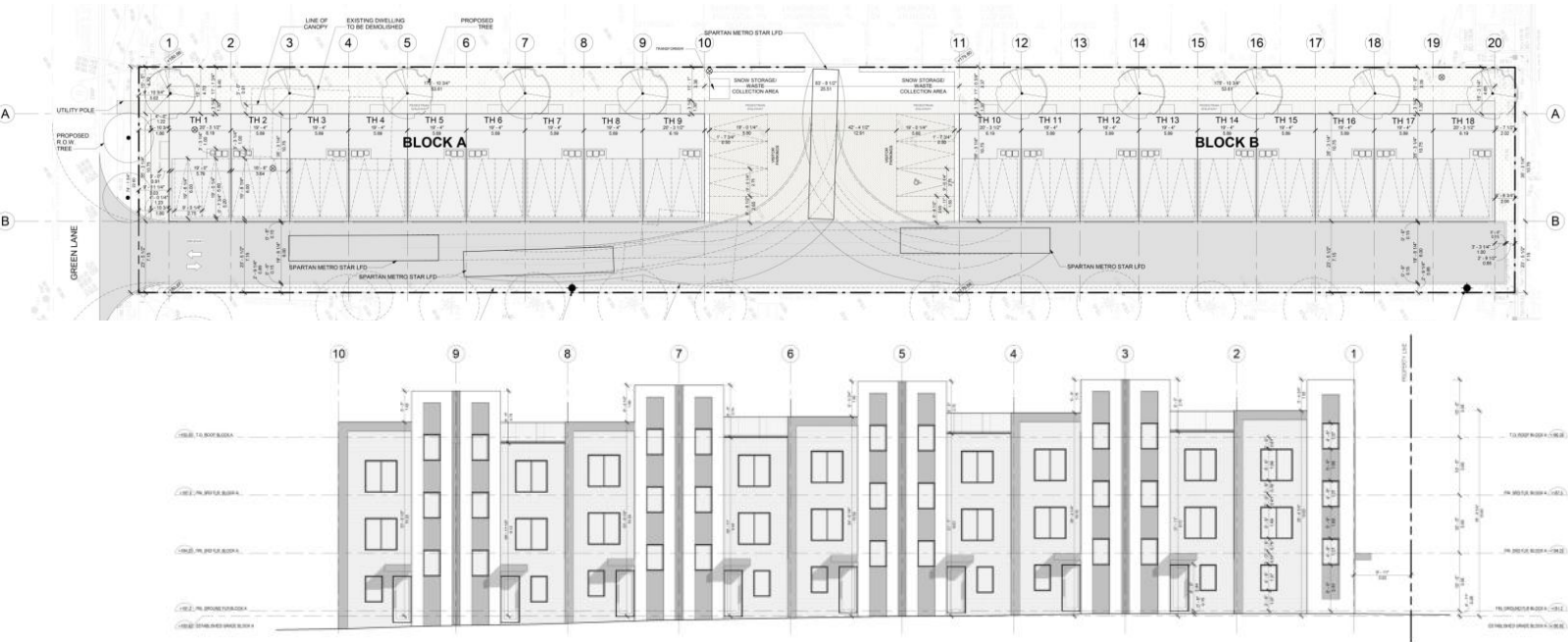
East Elevation
