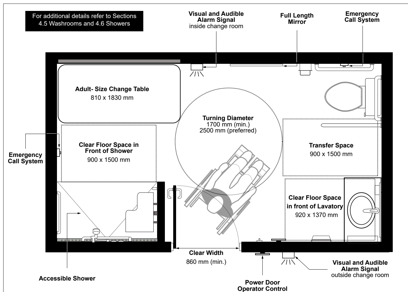
Figure 94: Universal Change Room
