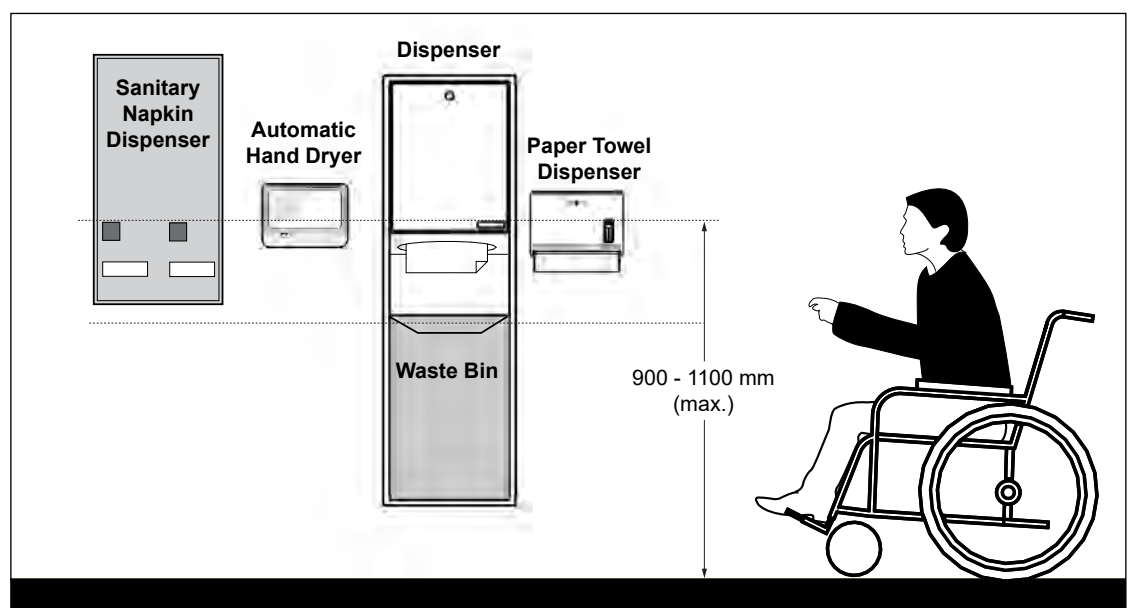
Figure 60: Typical Washroom Amenities
