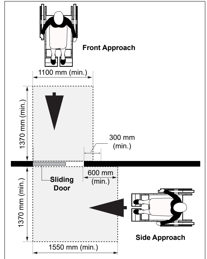
Figure 44d: Front and Side Approach at Sliding Door - Plan View
