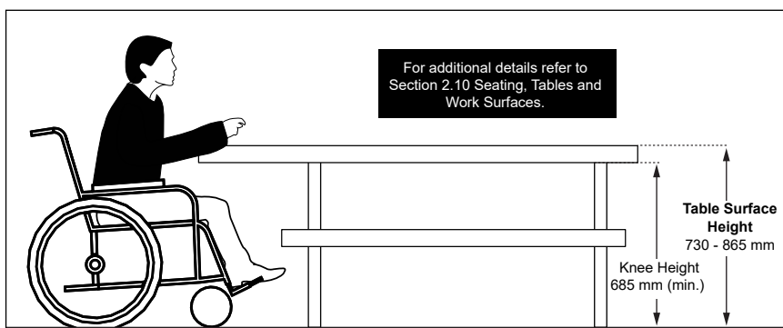
Figure 101b: Picnic Table Design and Features - Elevation View
