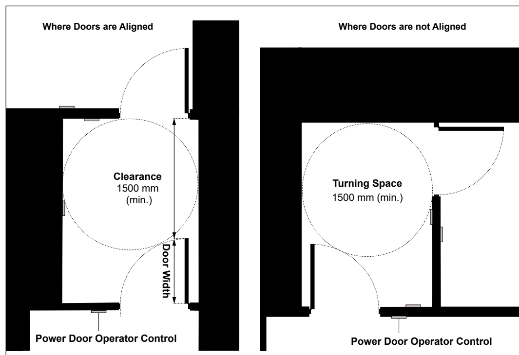
Figure 45: Doors in Series - Plan View
